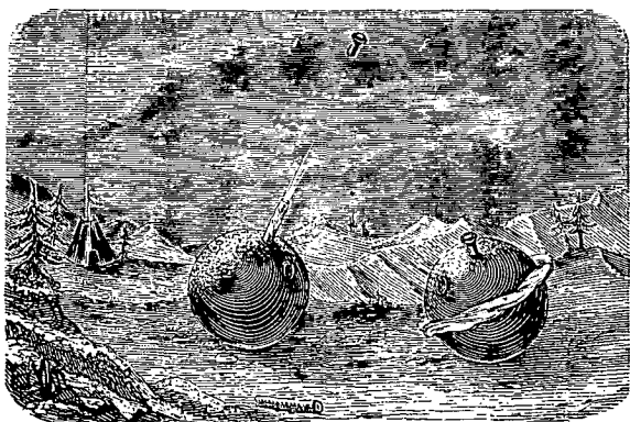
Fig. 64. — Force expansive de la glace.
