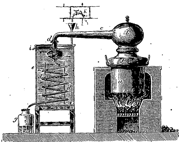
Fig. 75. — Alambic.
