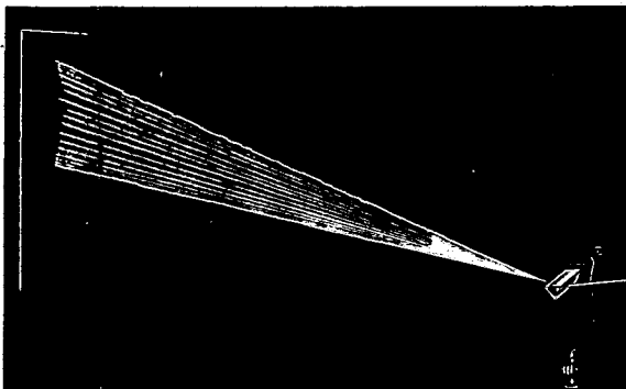
Spectre Solaire (Fig 29)
